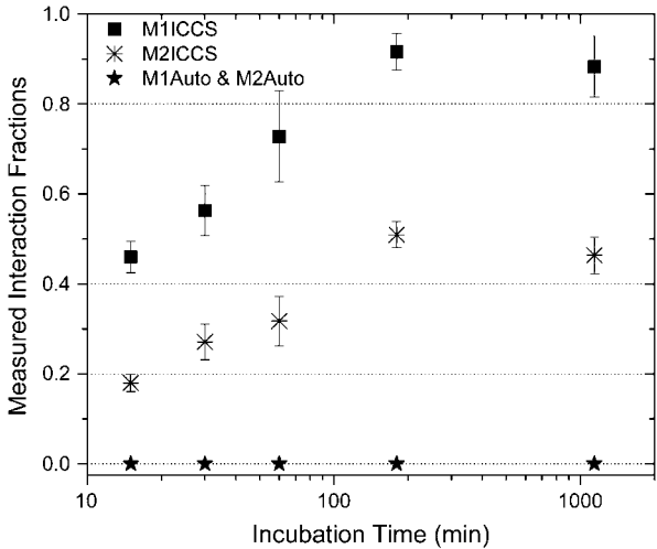
FIGURE 6 Plot of measured interaction fractions as a function of incubation time for a secondary FITC anti-mouse IgG (Fab-specific), and a secondary Alexa 633 anti-mouse IgG (Fc-specific) incubated on a coverslip coated with mouse monoclonal IgG. Each point is an average of 10 dual color image analyses recorded from different regions of the sample. Error bars are propagated standard errors of the mean.
