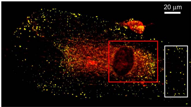
FIGURE 7 Two-channel overlay RGB image of PDGF- \beta receptors on human foreskin fibroblast cells immunolabeled with FITC (green) and Alexa-633 (red). The boxes indicate the regions chosen for colocalization analysis. Both methods lead to analogous results in the region indicated by the white box ( M1_{\text{ICCS}} = 0.98 , M2_{\text{ICCS}} = 1.0 , M1_{\text{Auto}} = 0.96 , and M2_{\text{Auto}} = 0.94 ). ICCS fails in the region indicated by the red box due to the edge boundaries of the nuclear region while automatic colocalization works well in this regime ( M1_{\text{Auto}} = 0.92 and M2_{\text{Auto}} = 0.35 ).
